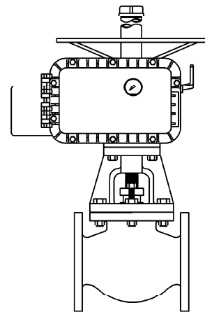
WITH ELECTRIC OPERATOR
