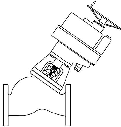
WITH ELECTRIC OPERATOR
